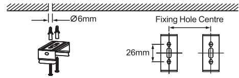
2. According to the Fixing hole centre, instal expansion bolts and screws, instal the bracket.
